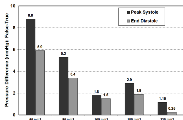
Fig. 6 Pressure difference between false and true lumina vs. total area of the tear sizes
