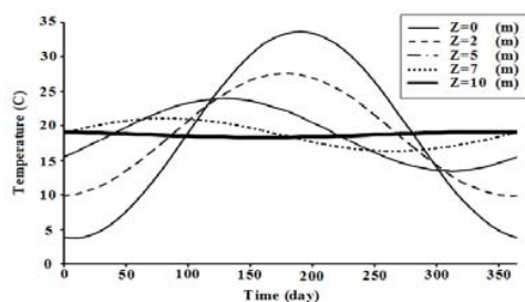
Fig. 2 Ground temperature profile at different depth
