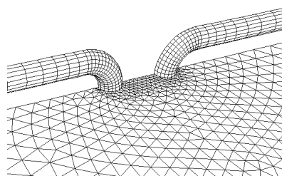
Fig.4 (a) Schematic of the computational grid in the symmetry plane of one borehole (b) Magnification of mesh neighboring to one borehole
