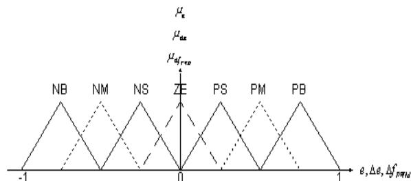
Fig. 3 Input and output Membership functions
