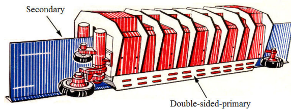
Fig. 1 Double-sided linear induction motor
