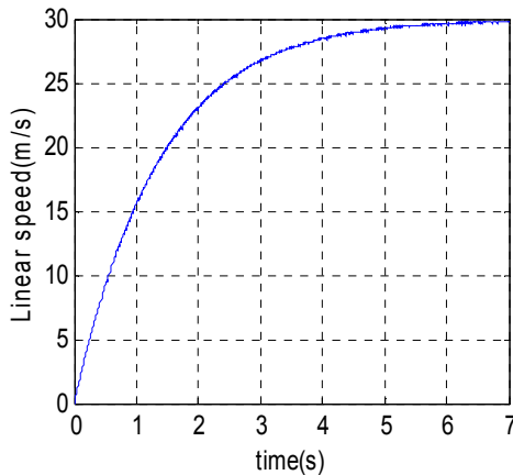
Fig. 15 Linear speed Vs time characteristic 8 poles motor
