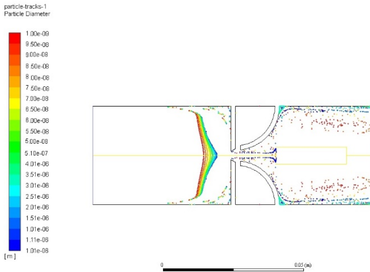
Fig. 8 Particle diameter
