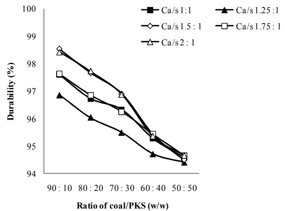
Fig. 4 Durability of bio-briquettes using scallop shell desulfurizer
