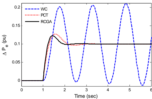
Fig. 6. Electrical power deviation response for Case-I
