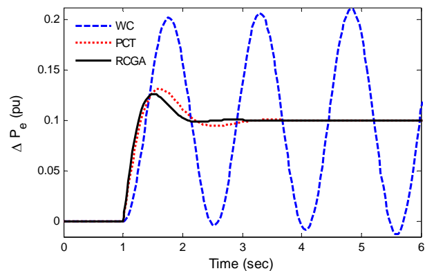
Fig. 8. Electrical power deviation response for Case-II
