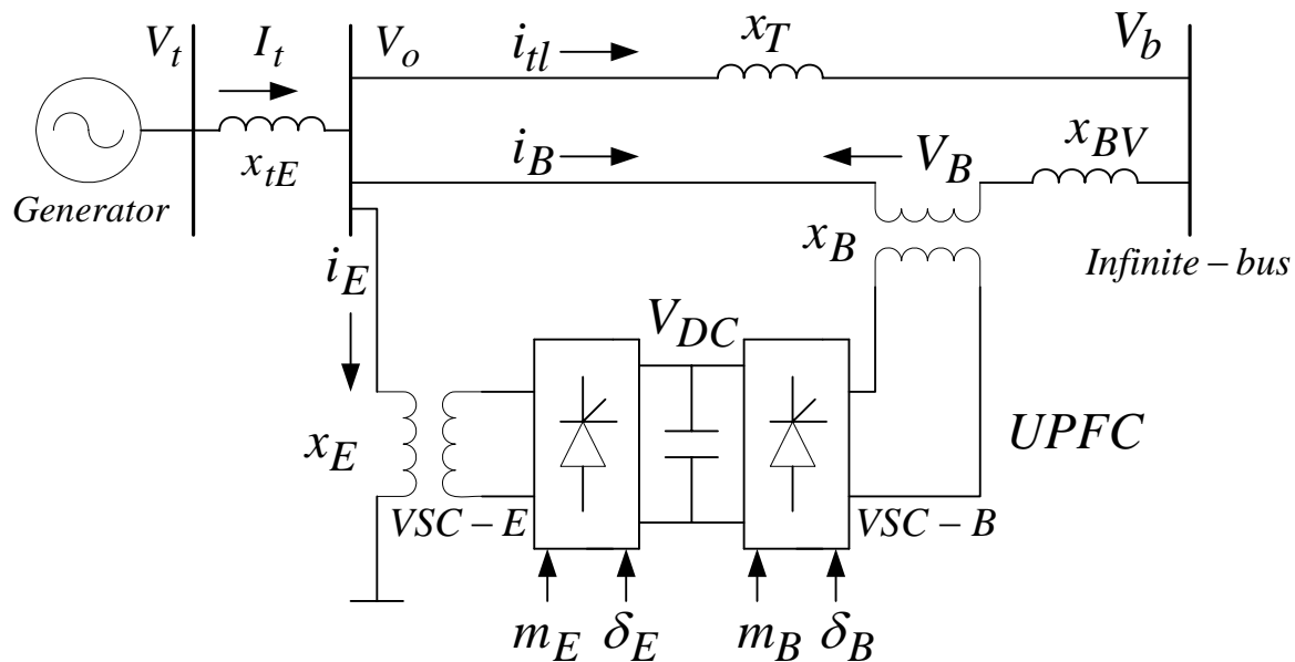
Fig. 1. Single-machine infinite-bus power system with UPFC
