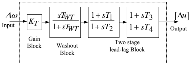
Fig. 3. Structure of the UPFC-based damping controller
