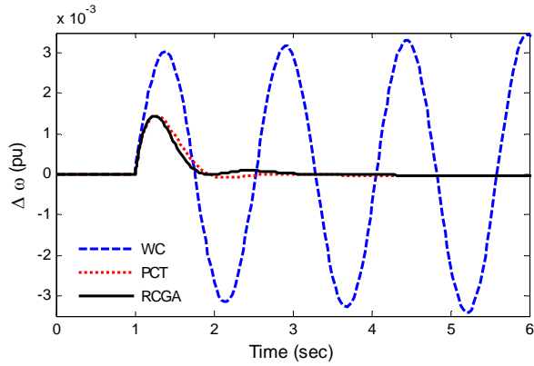
Fig. 9. Speed deviation response for Case-III
