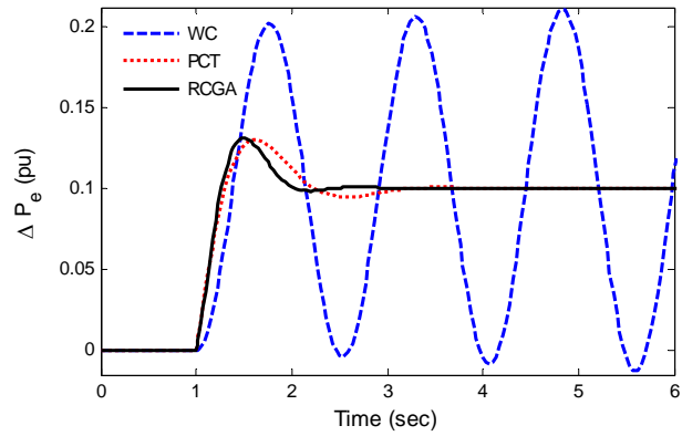
Fig. 12. Electrical power deviation response for Case-IV
