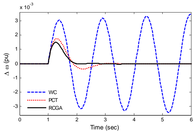
Fig. 7. Speed deviation response for Case-II
