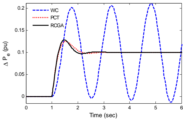
Fig. 10. Electrical power deviation response for Case-III
