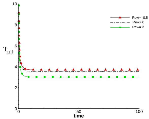
Fig. 6 Variations of viscous torque at the inner sphere with time for Re = 20 , \Omega_{oi} = 0
