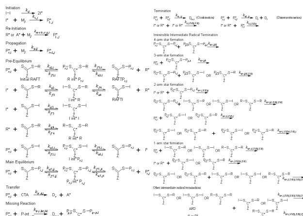
Scheme 1. Universal RAFT mechanism including probable side reactions
