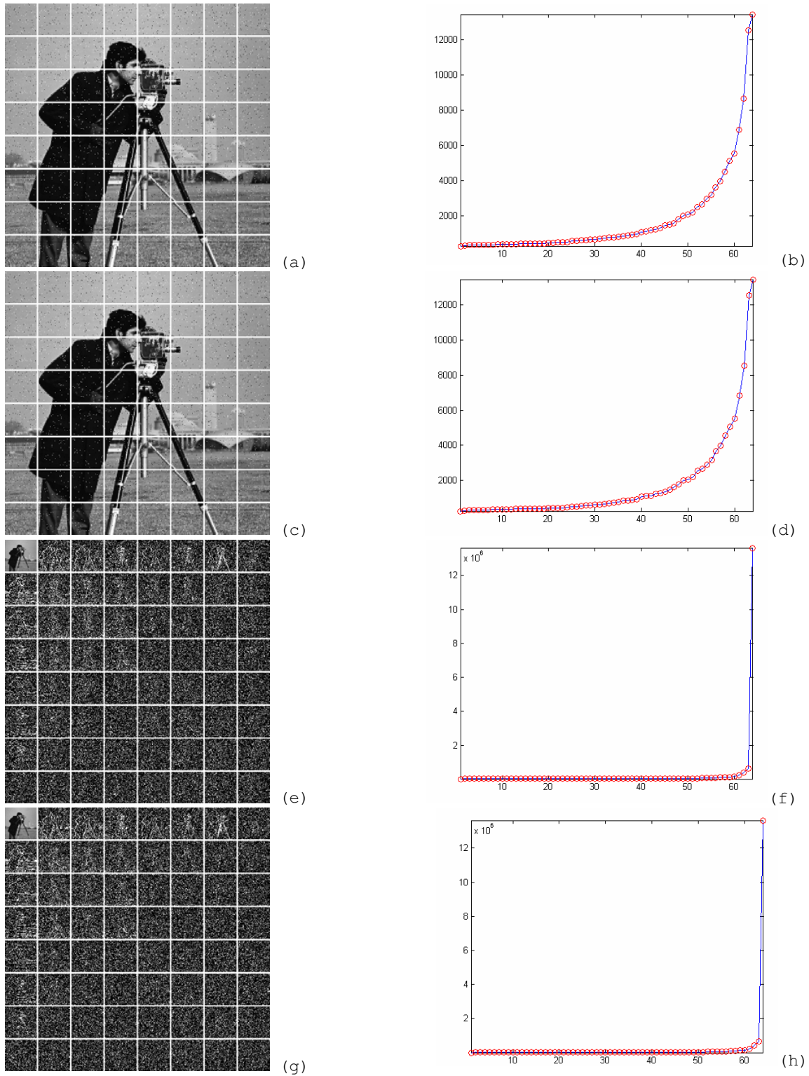
Fig. 17 Comparisson of efficiency: (a) sub-blocks set for Morton's scan + KLT, (b) eigenvalues distribution for Morton's scan + KLT, (c) sub-blocks set for row-rafter scan + KLT, (d) eigenvalues distribution for row-rafter scan + KLT, (e) sub-blocks set for Haar + Morton's scan + KLT, (f) eigenvalues distribution for Haar + Morton's scan + KLT, (g) sub-blocks set for Haar + row-rafter scan + KLT, and (h) eigenvalues distribution for Haar + row-rafter scan + KLT
