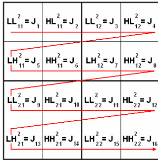
Fig. 13 Row rafter scanning
