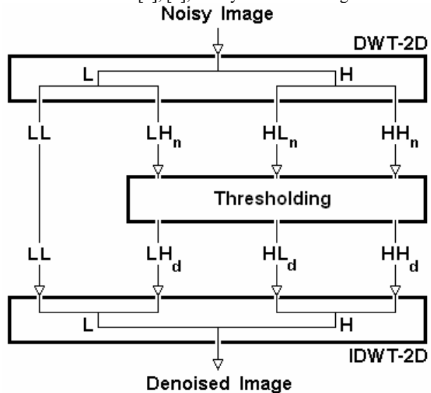
Fig. 4 Thresholding Techniques
