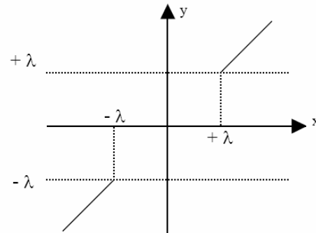
Fig. 5 (b): Hard-Thresholding
