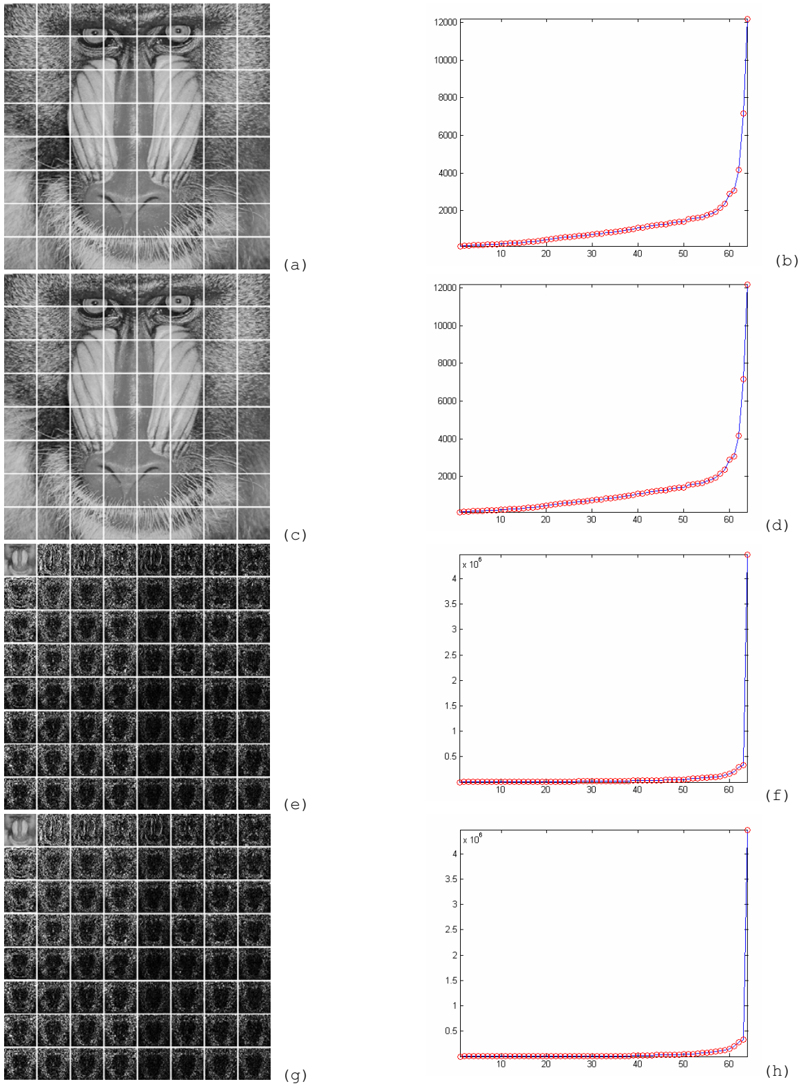
Fig.19 Comparisson of efficiency: (a) sub-blocks set for Morton's scan + KLT, (b) eigenvalues distribution for Morton's scan + KLT, (c) sub-blocks set for row-rafter scan + KLT, (d) eigenvalues distribution for row-rafter scan + KLT, (e) sub-blocks set for Haar + Morton's scan + KLT, (f) eigenvalues distribution for Haar + Morton's scan + KLT, (g) sub-blocks set for Haar + row-rafter scan + KLT, and (h) eigenvalues distribution for Haar + row-rafter scan + KLT
