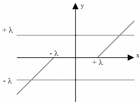
Fig. 5(a) Soft-Thresholding
