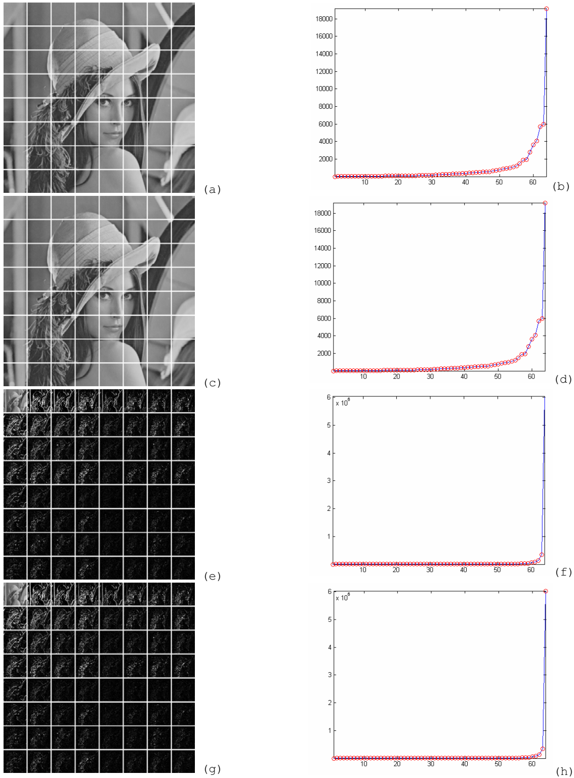
Fig. 15 Comparisson of efficiency: (a) sub-blocks set for Morton's scan + KLT, (b) eigenvalues distribution for Morton's scan + KLT, (c) sub-blocks set for row-rafter scan + KLT, (d) eigenvalues distribution for row-rafter scan + KLT, (e) sub-blocks set for Haar + Morton's scan + KLT, (f) eigenvalues distribution for Haar + Morton's scan + KLT, (g) sub-blocks set for Haar + row-rafter scan + KLT, and (h) eigenvalues distribution for Haar + row-rafter scan + KLT
