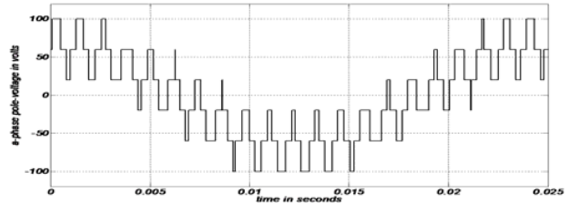
Fig. 8.a A-phase pole-voltage with f_1=40\text{Hz} .
