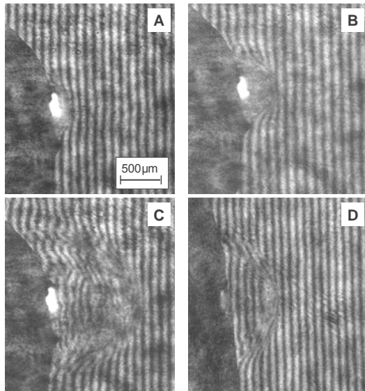
Fig. 2. Interferograms demonstrating dynamics of shock wave in water. A, B, C-laser pulse energy \varepsilon_{lp}=75 \text{ mJ} ; D- \varepsilon_{lp}=47 \text{ mJ} . Time delays:A-35; B-153; C-581 and D-484 ns
