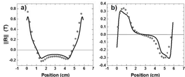
Fig. 4 Experimental (open dots) and theoretical (lines) values of the a) normal and b) tangential component of the magnetic field at the magnet surface of the unbalanced 2 configuration
