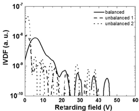
Fig. 7 IVDF for the three different magnetic configurations at a pressure of 5.10^{-3} mbar and 300W of discharge power
