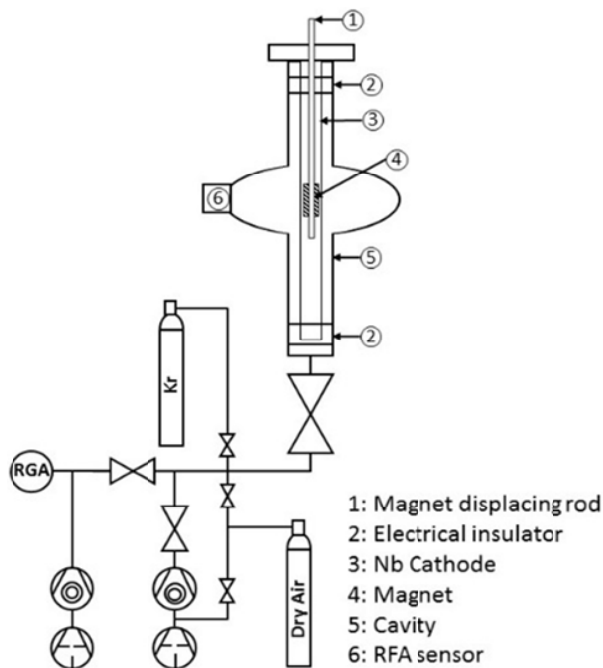
Fig. 2 Schematic of the SRF cavities coating apparatus
