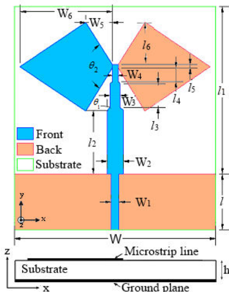
Fig. 1 UWB bowtie patch antenna geometry [6]
