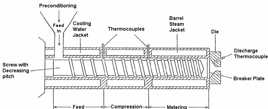
Fig. 1 Single-screw extruder
