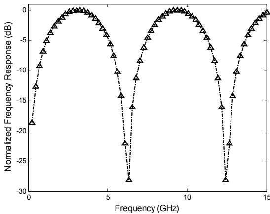
Fig. 4 Frequency responses of the two-tap microwave bandpass filter for L_1-L_2=1.6 cm, \Delta\tau_d=0 ps, \text{FSR}=6.25 GHz
