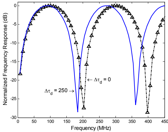
Fig. 3 Frequency responses of the two-tap microwave bandpass filter for L_1-L_2=0.5 m, \Delta\tau_d=250 ps, \text{FSR}=181.81 MHz; \Delta\tau_d=0 ps, \text{FSR}=200 MHz
