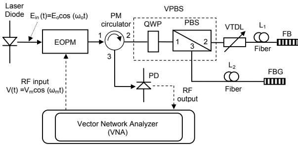
Fig. 1 Block diagram of the microwave bandpass filter
