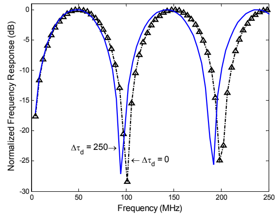
Fig. 2 Frequency responses of the two-tap microwave bandpass filter for L_1 - L_2 = 1 m, \Delta\tau_d = 250 ps, FSR=95.24 MHz; \Delta\tau_d = 0 ps, FSR=100 MHz
