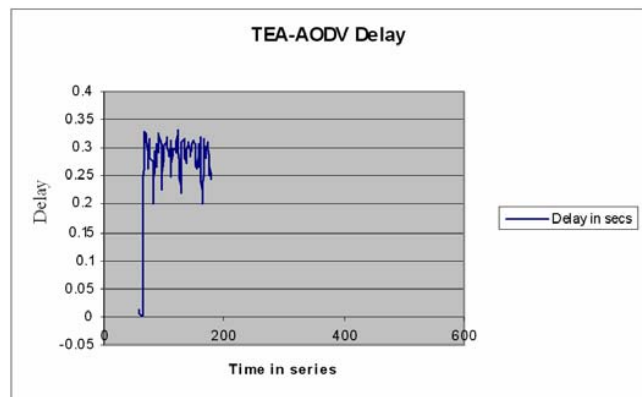
Fig. 2 TEA-AODV Delay
