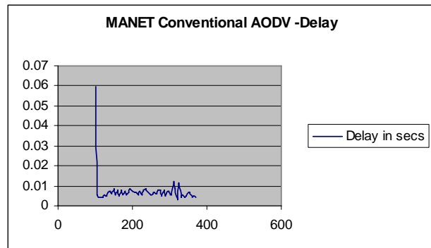
Fig. 1 AODV Delay
