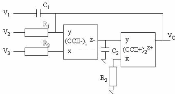
Fig. 2. Circuit diagram of the proposed voltage-mode triple-input single-output multifunction filter.
