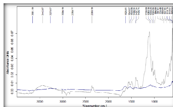
Fig. 8 FTIR spectrum of untreated and treated sample containing of Reactive red 195 (50 ppm)
