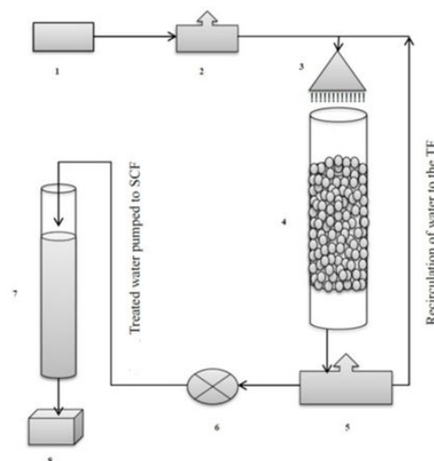
Fig. 1 Schematic diagram of treatment process, where; 1. Sedimentation Tank for untreated wastewater, 2. Plastic container with water pump, 3. Shower rose, 4. FBR filled with stone media, 5. Plastic container with water pump, 6. Peristaltic pump, 7. Sand column Filter, 8. Treated water
