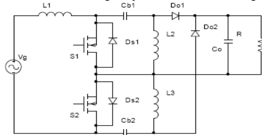
Fig. 3 Bridgeless SEPIC AC-DC converter [11]
