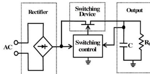
Fig. 5 AC-DC converter by chopping input [12]
