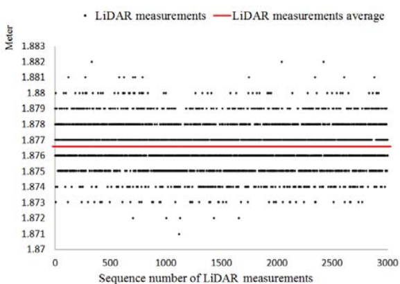
Fig. 10 Accuracies of LiDAR distance measurements
