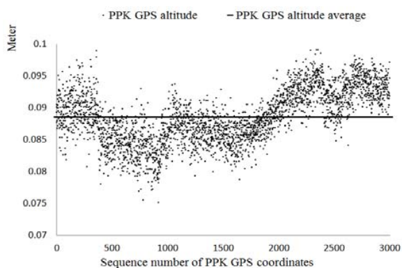
Fig. 9 Accuracies of PPK GPS altitude
