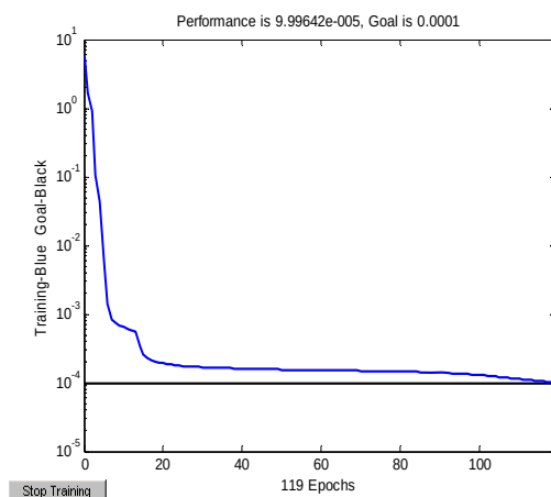
Fig. 6 ANN training performance
