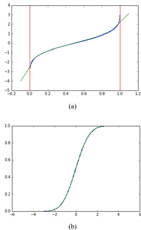
Fig. 2 (a) 2-layer with 100 \times 100 nodes with 1 input variable; (b) 1-layer with 100 nodes with 3 input variables. Curve line: inverse CDF from U(0,1) (x-axis) to N(0, 1) (y-axis), Dotted piecewise linear line: spline approximation trained by GAN
