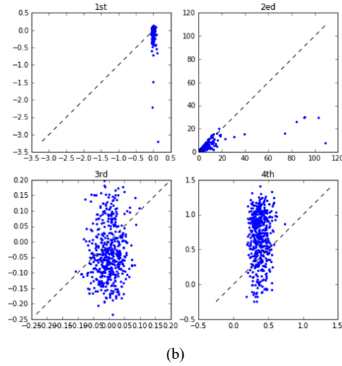
Fig. 13 Mean (1st), variance (2nd), skewness (3rd) and kurtosis (4th) between the generated conditional distributions (y-axis) and the true ones (x-axis); (a) for \text{CGAN}_{\sigma_t} and (b) for \text{CGAN}_{\sigma_{t-1}}
