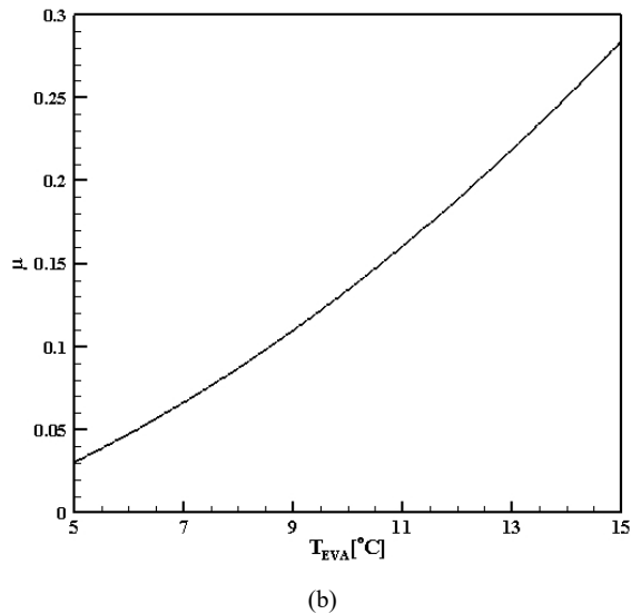
Fig. 10 Effect of evaporator temperature on the entrainment ratio
