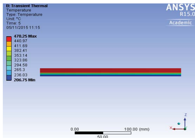
Fig. 5 Temperature distribution on the plates
