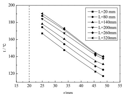
Fig. 4 Steady-state radial temperature distribution
