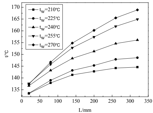
Fig. 9 Effect of t_w on axial temperature distribution
