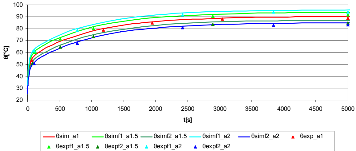
Fig. 9 Maximum fuse links temperature time evolution for current value of 160A and different asymmetry coefficient a = 1; 1.5; 2 . Comparison between simulation ( \theta_{sim\_a1} , \theta_{simf1\_a1.5} , \theta_{simf1\_a2} , \theta_{simf2\_a1.5} , \theta_{simf2\_a2} ) and experimental values ( \theta_{exp\_a1} , \theta_{expf1\_a1.5} , \theta_{expf1\_a2} , \theta_{expf2\_a1.5} , \theta_{expf2\_a2} )
