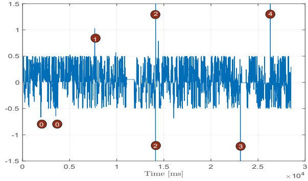
Fig. 9 Real-time lateral error sample data obtained during the 60km tour on M40 highwa- Madrid. The data demonstrating the undetectable lane marks on the road, cases 2,3, and 4
