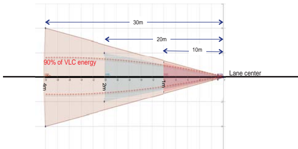
Fig. 8 The three main zones where the VLC receiver was placed to evaluate the received signal level. The experiment was conducted with respect to the variation of direct distances changes and out-door conditions
