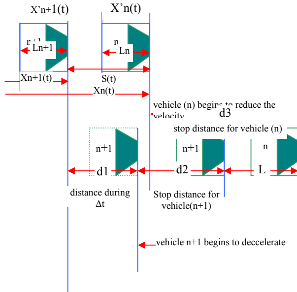
Fig. 3 Vehicle position approaching stop line
