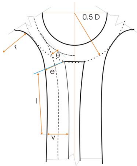
Fig. 2 Roundabout Geometry
