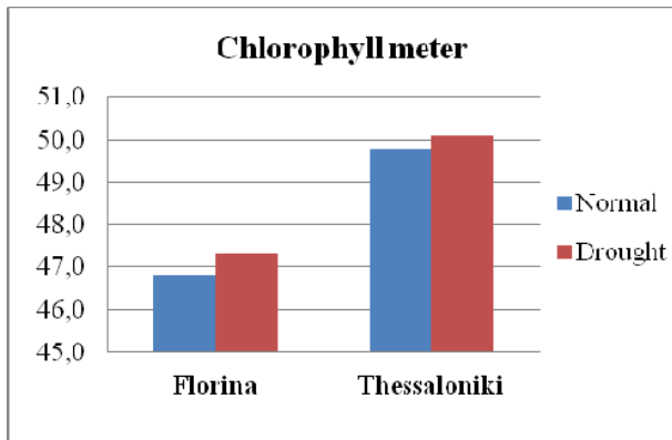
Fig. 6 Chlorophyll meter readings (SPAD) at two locations (Florina and Thessaloniki) and two treatments, fowl water (normal) and 60% water (drought)
