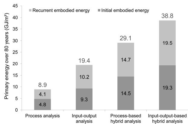
Fig. 3 Life cycle embodied energy demand of the case study passive house, by embodied energy quantification technique, per m² of usable floor area. Note: figures may not sum due to rounding
