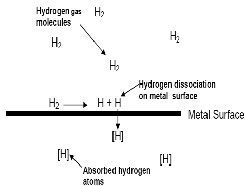
Fig. 1 Hydrogen adsorption in metals exposed to a gaseous Hydrogen environment
