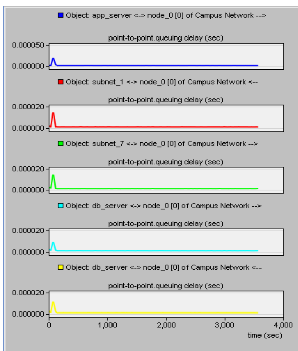
Fig. 16 Queuing delay point to point objects
