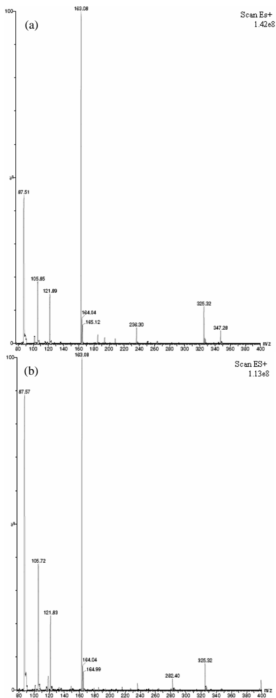
Fig. 4 Mass spectrometry of methomyl degradation of at the reaction time of (a) 0 minute, and (b) 30 minutes, by Fenton reagents \text{H}_2\text{O}_2 and \text{Fe}^{2+} of 1.0 mM and 0.5 mM, respectively
