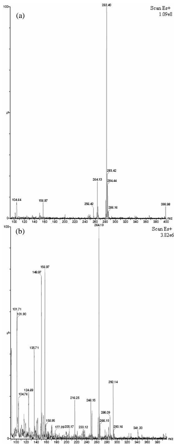
Fig. 5 Mass spectrometry of parathion degradation of at the reaction time of (a) 0 minute, and (b) 30 minutes, by Fenton reagents \text{H}_2\text{O}_2 and \text{Fe}^{2+} of 1.0 mM and 0.5 mM, respectively
