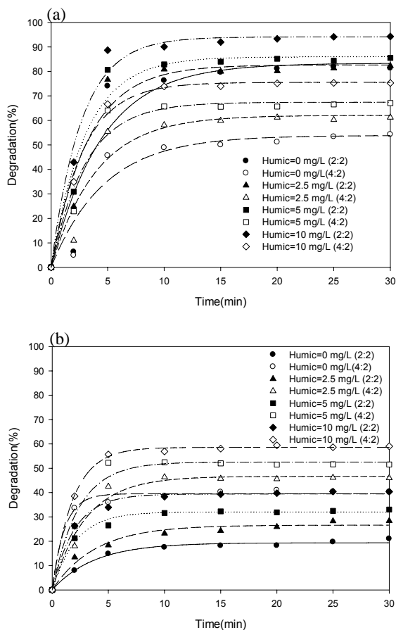
Fig. 3 Methomyl (a) and parathion (b) degradation at the presence of humic acid concentrations of 2.5, 5 and 10 mg/L, the \text{H}_2\text{O}_2 to \text{Fe}^{2+} concentration ratio of 4:2 and 2:2
