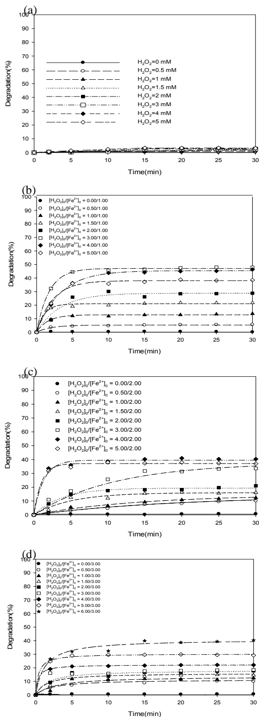
Fig. 2 Parathion degradation at various Fenton reagent dosage of \text{Fe}^{2+} concentration at (a) 0 mM, (b) 1 mM, (c) 2 mM and (d) 3 mM
