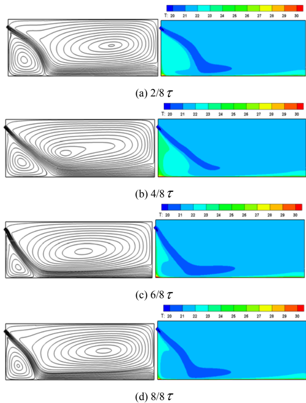
Fig. 3 Streamlines (left) and temperature contour (right) ( Am= 15^\circ, St= 5 \times 10^{-4} )
