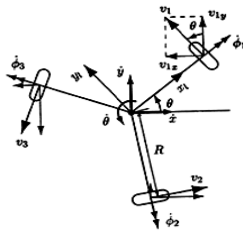
Fig. 1 Kinematics model of omnidirectional wheels[7]
