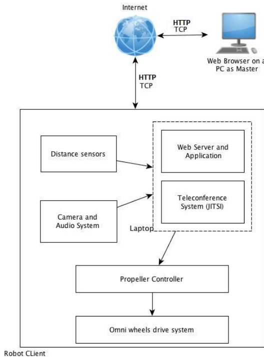
Fig. 2 Interconnecting Robot Client to Master through Internet
