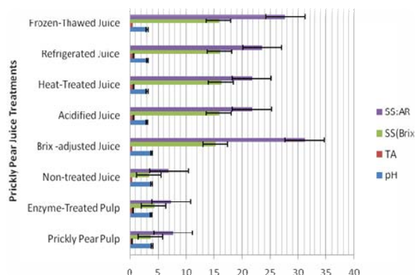
Fig. 1 Physicochemical Parameters of Prickly Pear Juices
