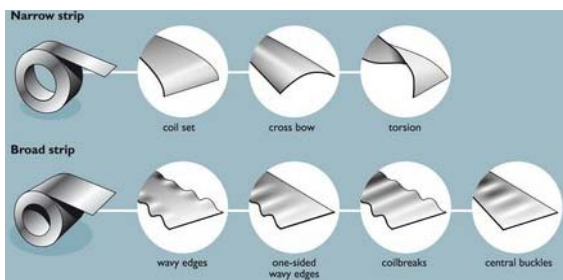
Fig. 1 Typical coil defects
