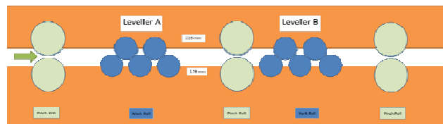
Fig. 14 While rolled mill machine in the manufacturing process consists of two roller set is set Leveler A and Leveler B
