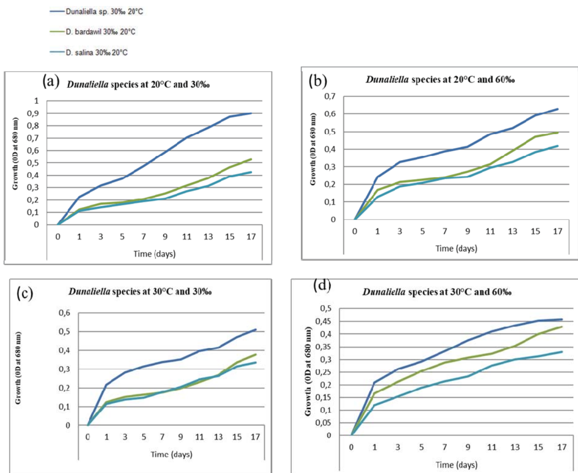
Fig. 3 Comparison of growth of three of Dunaliella species ( Dunaliella sp. , Dunaliella bardawil , and Dunaliella salina ) in cultures maintained under four different treatment combinations of 2 temperatures and 2 salinities: (a) 20°C/30‰; (b) 20°C/60‰; (c) 30°C/30‰, and (d) 30°C/ 60‰
