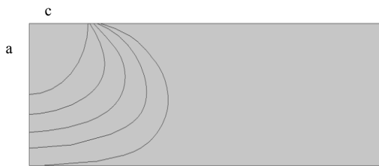
Fig. 9 The crack shape development for a deep semi-circular surface crack ( a/w=0.5, a/c=1 ) under ductile tearing in tension.
