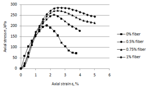
Fig. 4 Results of the unconfined compression tests
