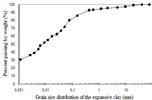
Fig. 1 Granulometric curve of the expansive clay
