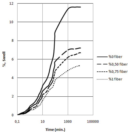
Fig. 6 Variation of percent swell of unreinforced and reinforced soil samples with time
