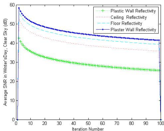
Fig. 4 Average SNR in winter's day, clear sky
