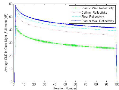
Fig. 2 Average SNR in clear night, full moon
