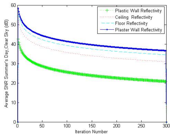
Fig. 6 Average SNR in summer's day, clear Sky
