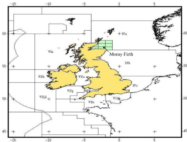
Fig. 1 Location of study area: The axis labels show latitude (degrees North) and longitude (degrees East). Green rectangles were used to calculate the habitat area in the Ecopath model
