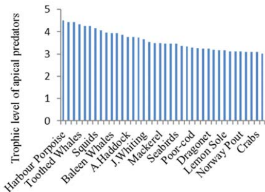
Fig. 2 Trophic level (TL) estimates of predators with TL ≥ 3.0 in Moray Firth ecosystem food web (in descending order)
