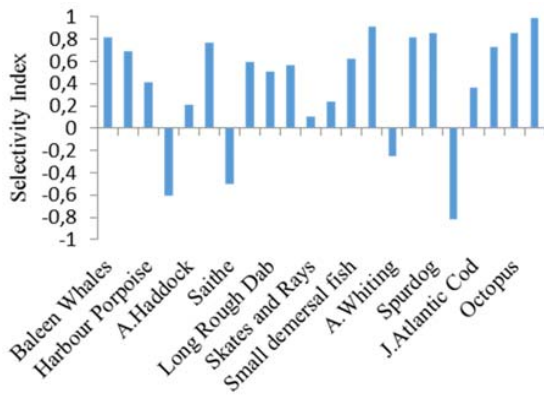
Fig. 6 showing the selectivity index (i.e. the degree of squid preference by its predators in the Moray Firth ecosystem) (A = adult, J = juvenile)
