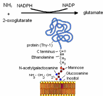
Fig. 1 The scheme of attachment of GPI protein to the PI membrane.
