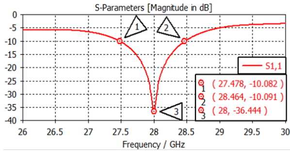
Fig. 2 Return loss of single element antenna
