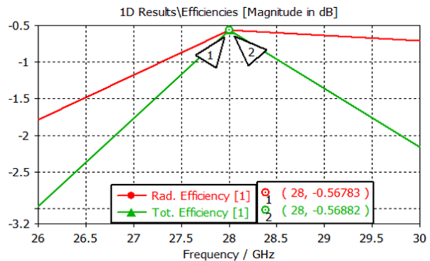
Fig. 5 Radiation and total efficiency of single antenna
