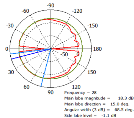
Fig. 8 (b) Array gain polar radiation on azimuth plane
