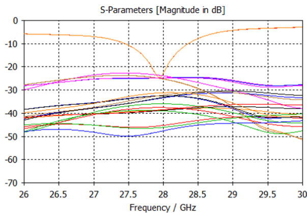
Fig. 7 Port isolations S11, S21, S31, etc.
