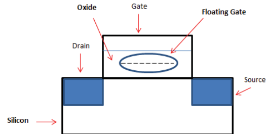
Fig. 3 Floating Gate
