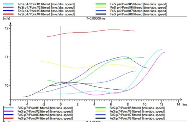
Fig. 4 FeSi grains velocity changings for the following pneumatic parameters: p_1 = 0.1 MPa and various p_4 , p_4 = 0.02, 0.04 and 0.06 MPa (analogically to fig. 3)
