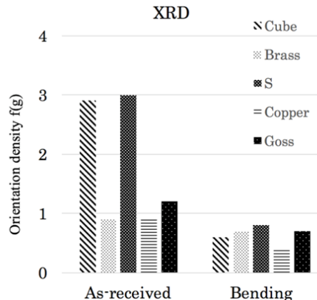
Fig. 7 Quantitative results of texture by XRD
