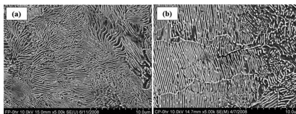
Fig. 3 Microstructures obtained by heat treatment for (a) fine pearlite (FP) and (b) coarse pearlite (CP) specimens
