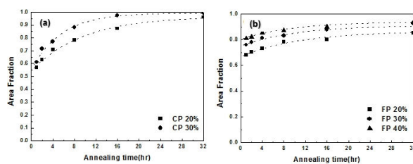
Fig. 5 Fraction of spheroidization as a function of annealing time obtained for FP and CP specimens with various cold reductions.
