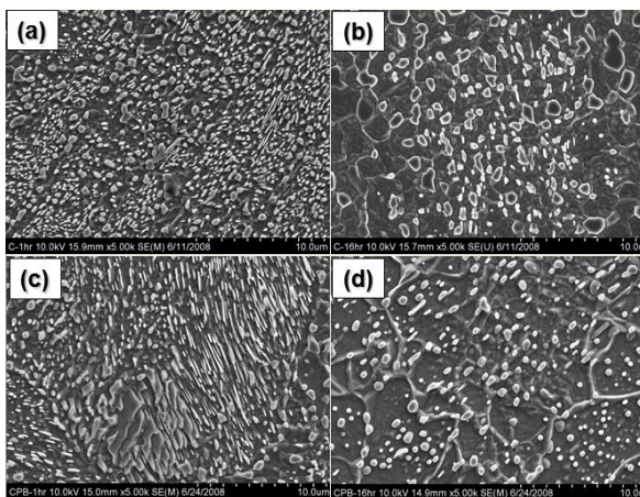
Fig. 4 Appearances of cementites of some selected specimens during spheroidization heat treatment taken from the 40%-cold-rolled FP specimen annealed for 1 hr (a) and 16 hrs (b), and the 30%-cold-rolled CP specimen annealed for 1 hr (c) and 16 hrs (d) at 720°C
