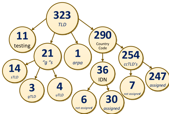
Fig. 3 Distribution of Top Level Domains (TLD)
